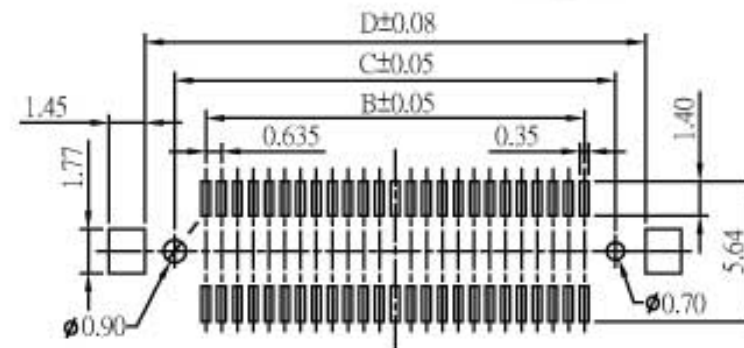
Recommended PCB Layout (PCB TOLERANCE ±0.05)
